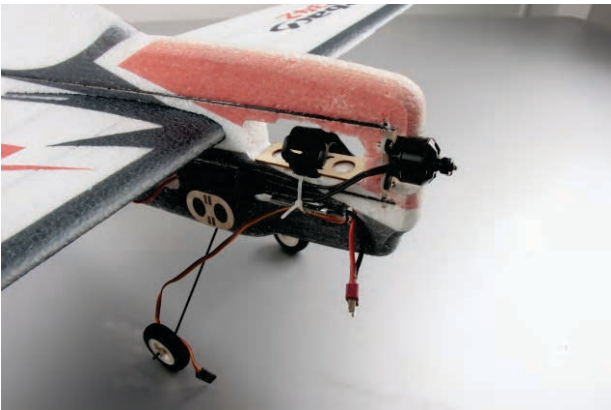
30. Connect motor and ESC, then adjust to correct motor running direction before flying. Put ESC into the slot of downside fuselage.
