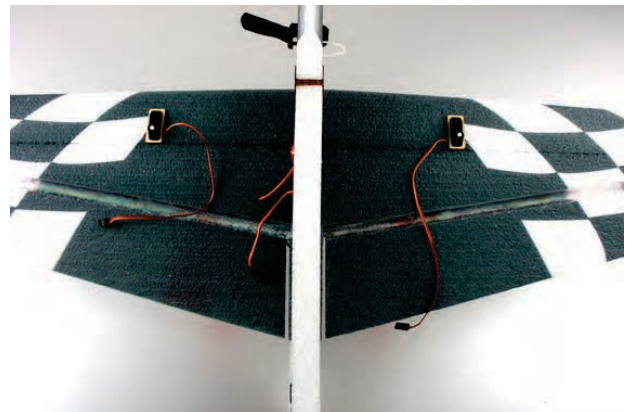
11. Put the servo into the pre-cut servo hole, then use glue to fix the servo mount onto the wing.
