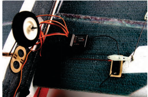
32. Link the servo leads and ESC to receiver, then test.
