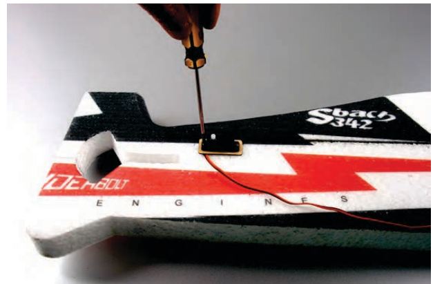
6. Embed servo leads into the slot.
