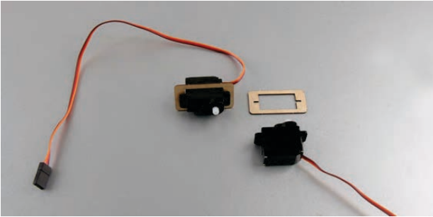
1. Install elevator servo into the servo mount.
