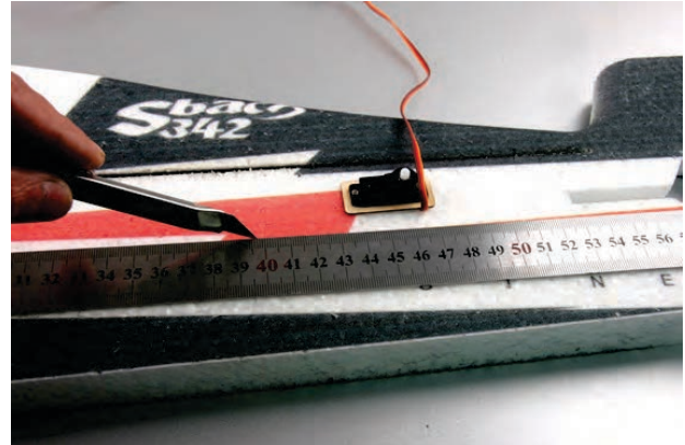
5. Cut a 10mm length slot on fuselage along a ruler, and make sure servo wire can be embedded deeply into the foam.
