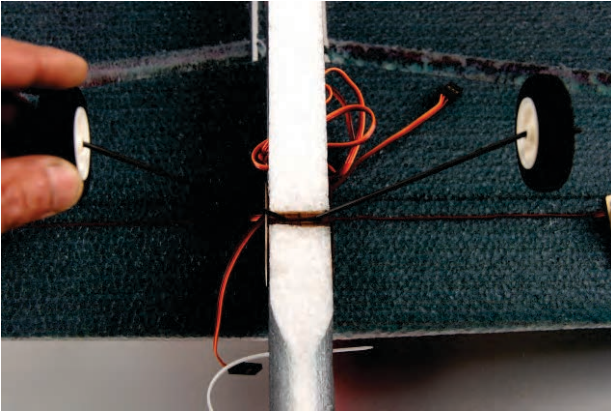
28. Insert landing gear frame into the slot on bottom fuselage, please refer to picture.
