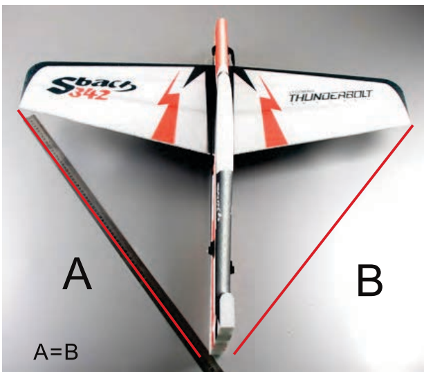
8. Insert the wing into the slot of fuselage and use glue to fix. Make sure A=B (refer to above picture).
