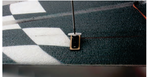
20. Fix servo arm extension on servo arm with 2pcs 2*4mm self tapping screws.
