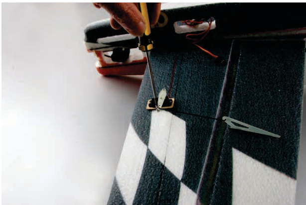
25. Put one end of steel wire into the hole of adjustor, then fix with screwdriver.
